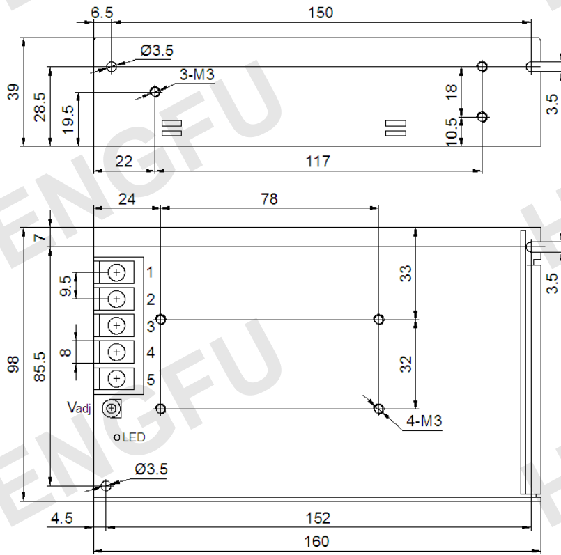
Terminal Pin No. Assignment 接线端子排布:
